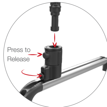
RAP-AAPUDU RAM® Universal Adapt-A-Post™ 4-Hole Drill-Down Base
