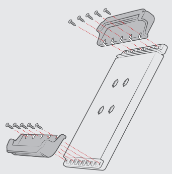
Interchangeable cups support any tablet
