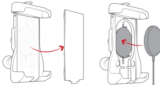
Removable backing plate to adjust the position of the Apple MagSafe charger
