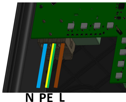
Fig. 15 Power supply connection detail
